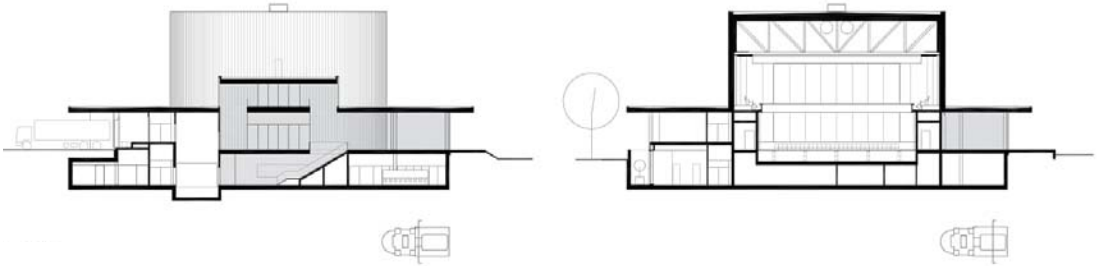
Cross sections
