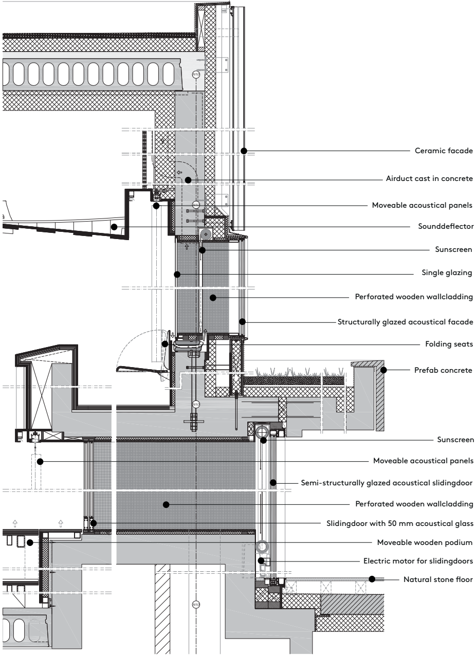
Section Facade Concerthall
